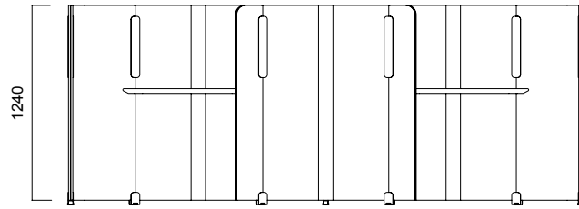
Tip 7 İkili Petek Panel
