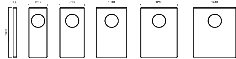
Kiss Panel H167 Pencereli
